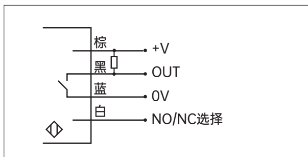
NPN NO+NC
