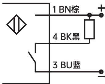
NPN 常开 (NO)
