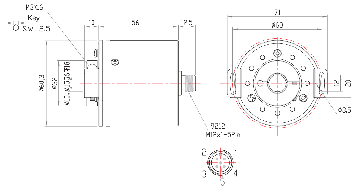
FDCE58B-CANopen+8138E+9212
