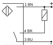
NPN-Normally open
