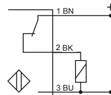
PNP-Normally closed
