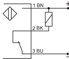
NPN-Normally closed
